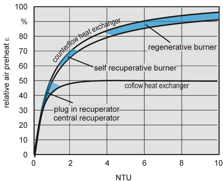
Figure 2: Heat exchanber performance
